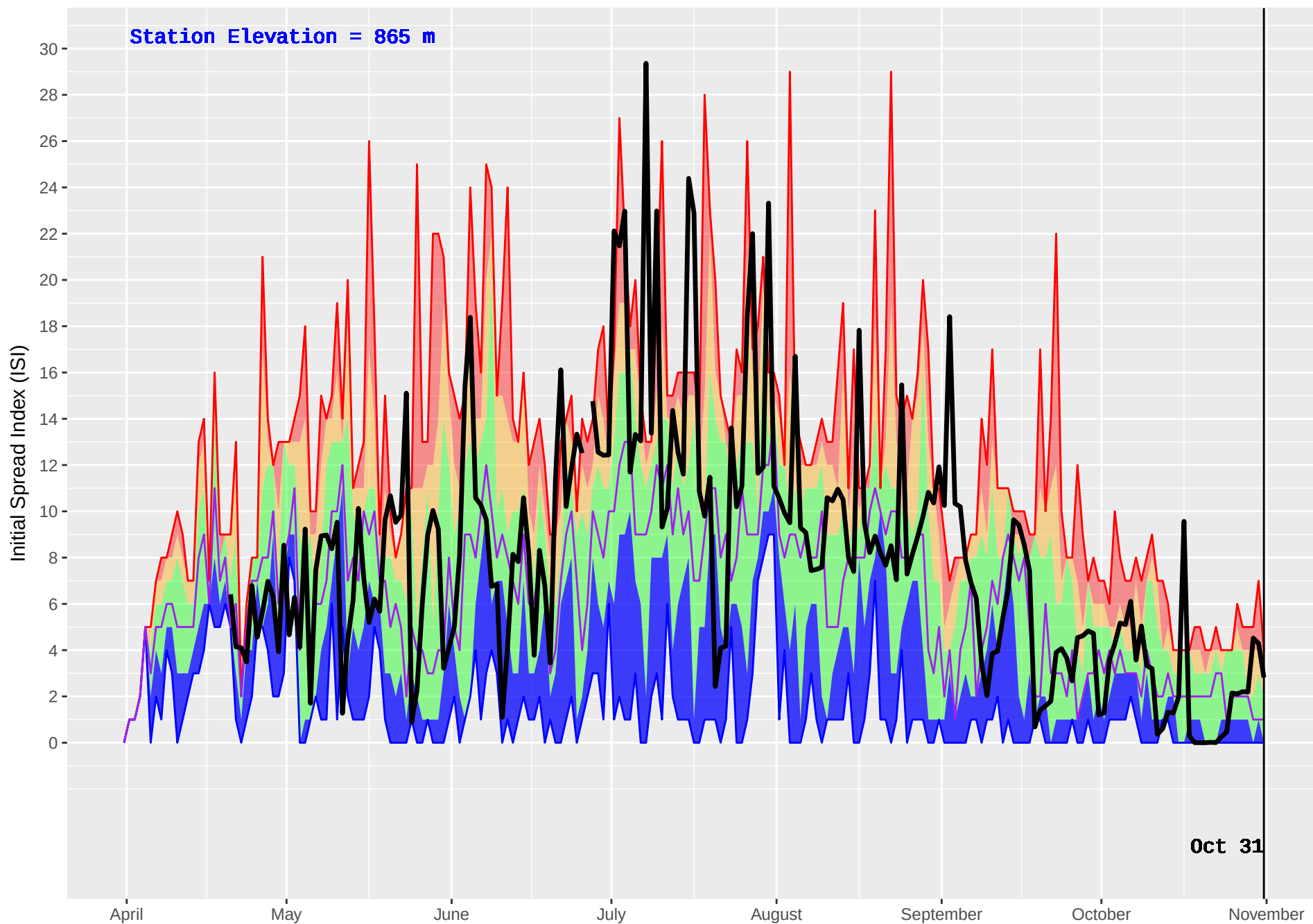
FIVE MILE (1029) : Historical (2008–2016) and Current (2017) Noon Initial Spread Index (ISI)
