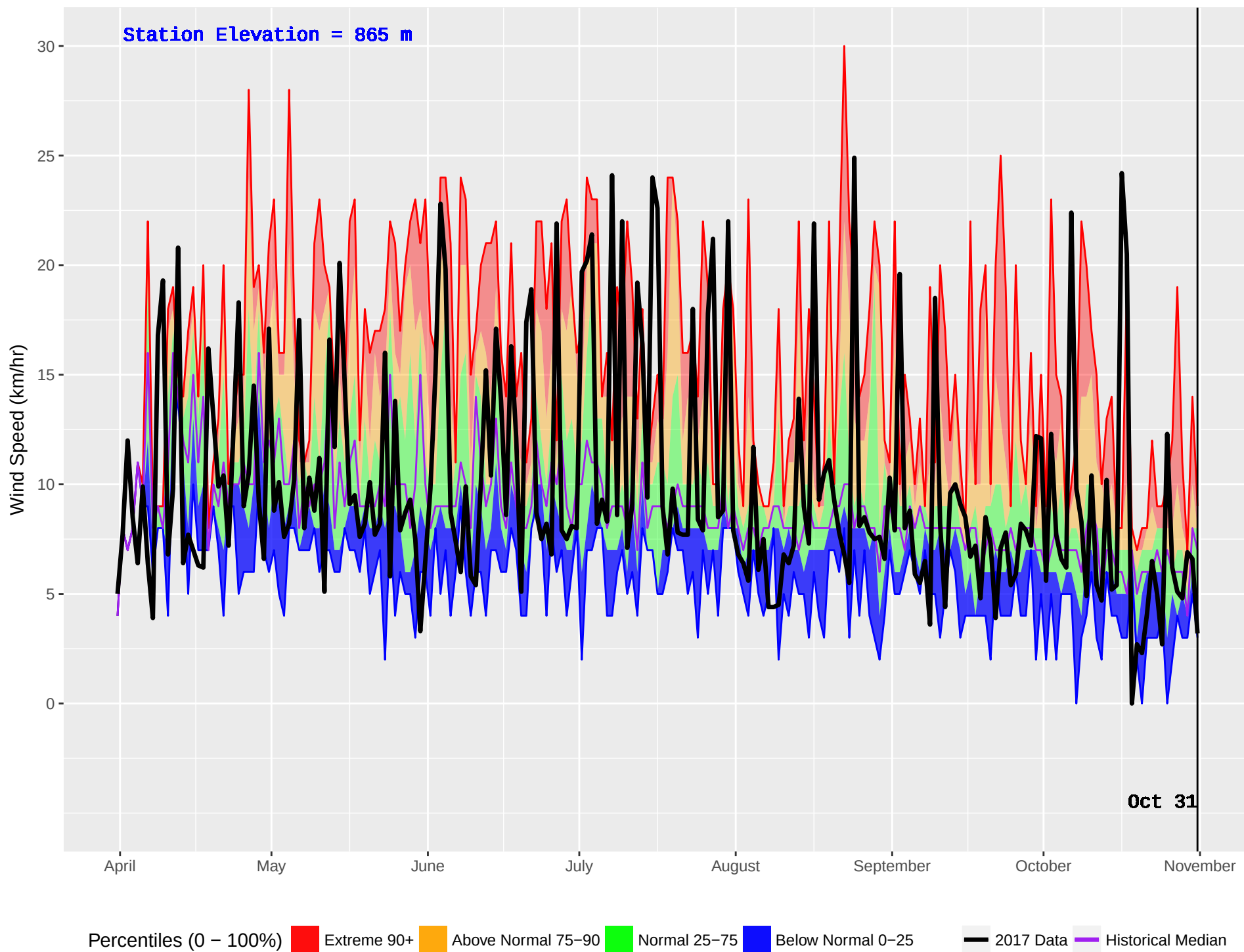
FIVE MILE (1029) : Historical (2008–2016) and Current (2017) Noon Wind Speed
