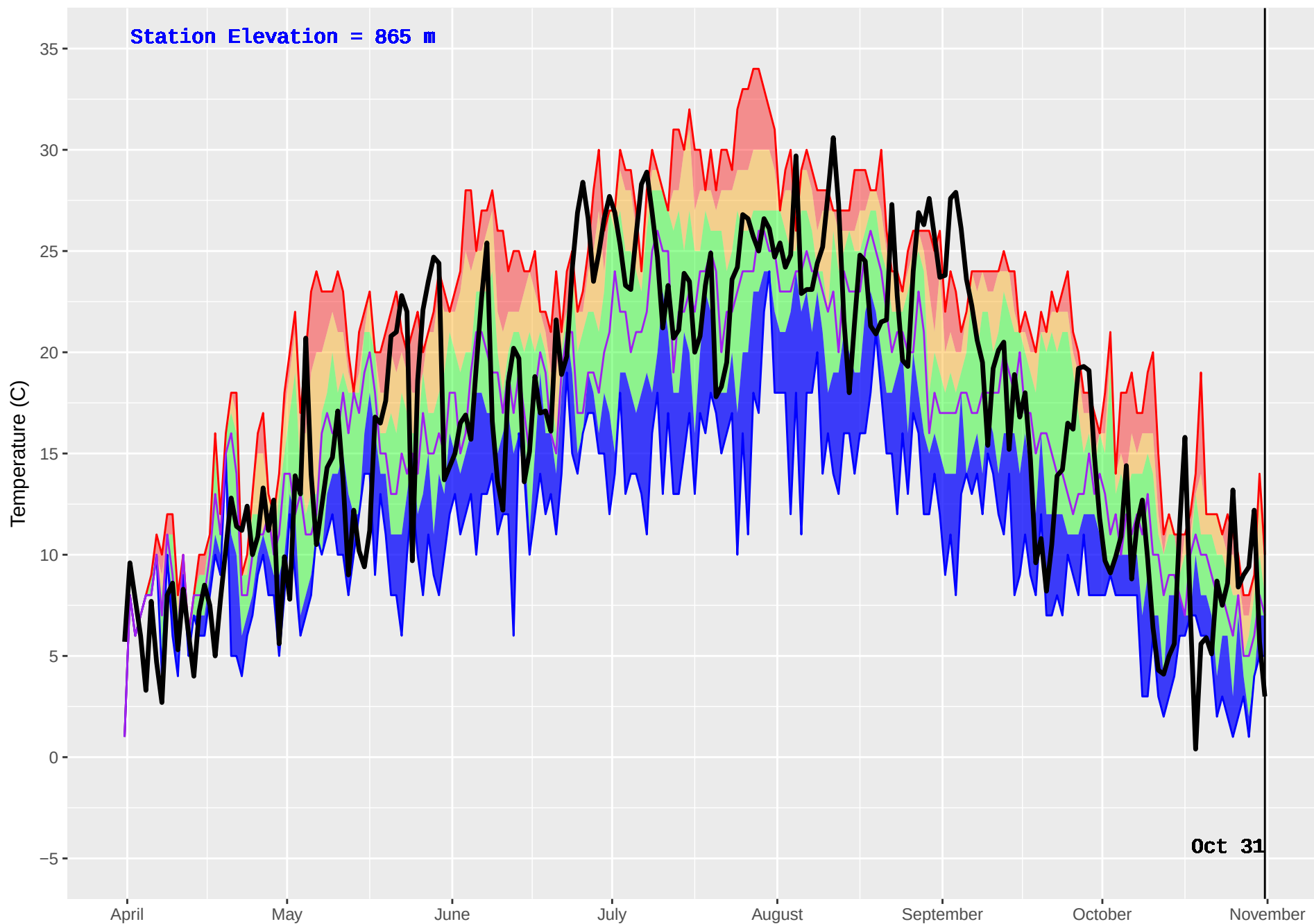
FIVE MILE (1029) : Historical (2008–2016) and Current (2017) Noon Temperature
