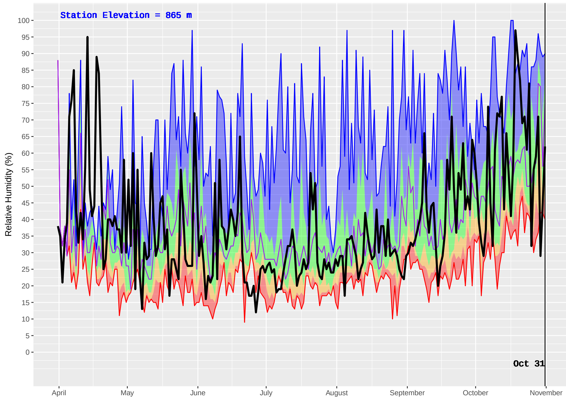
FIVE MILE (1029) : Historical (2008–2016) and Current (2017) Noon Relative Humidity
