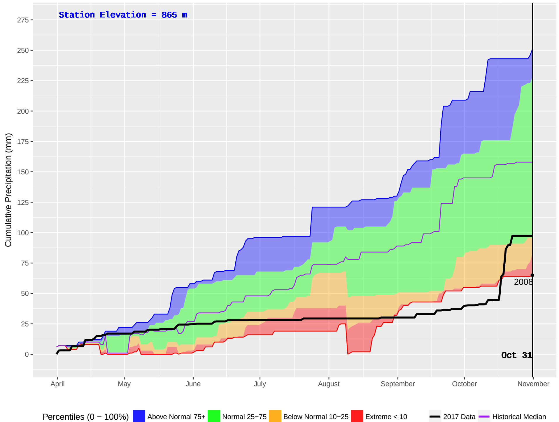
FIVE MILE (1029) : Historical (2008–2016) and Current (2017) Noon Cumulative Precipitation
