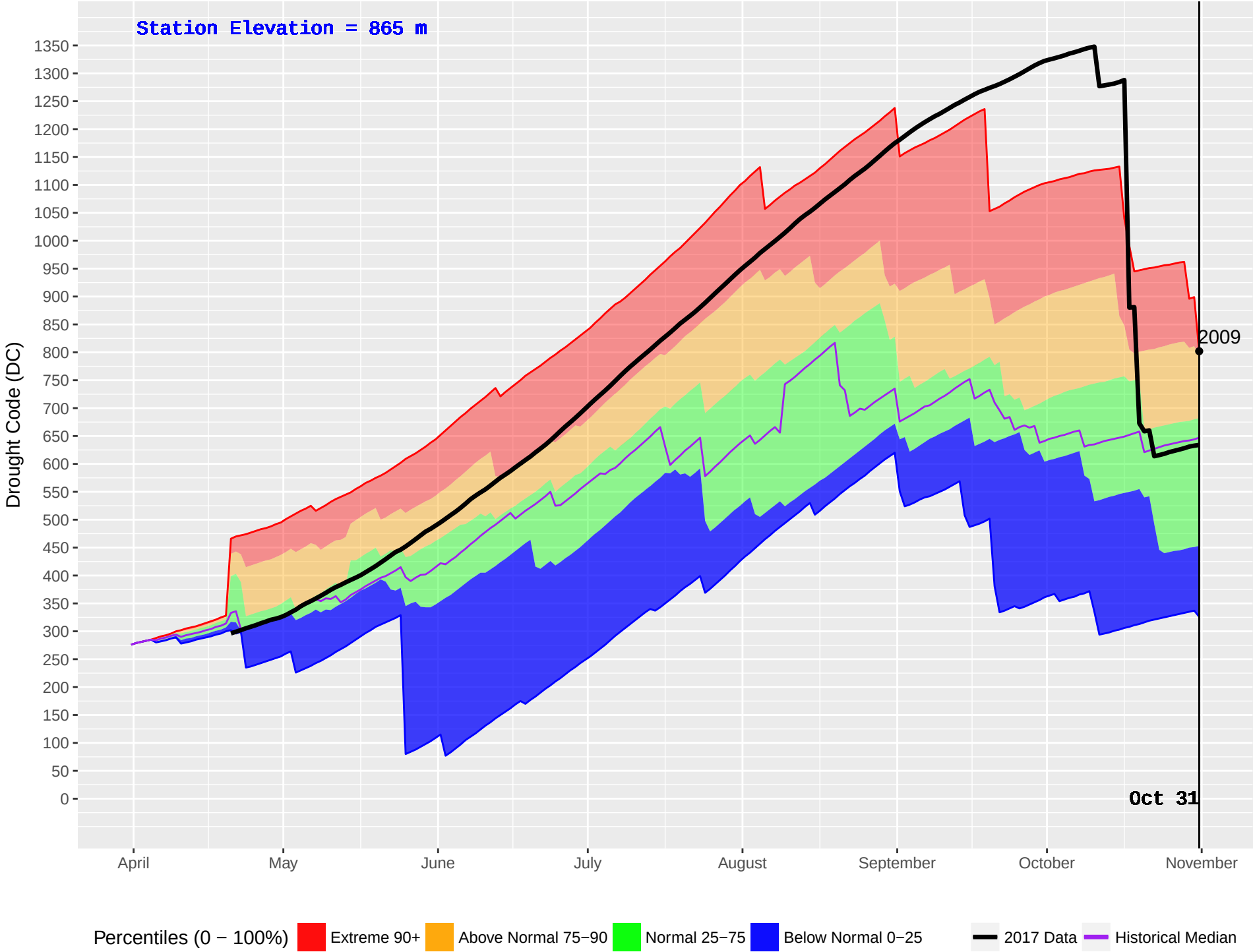
FIVE MILE (1029) : Historical (2008–2016) and Current (2017) Noon Drought Code (DC)
